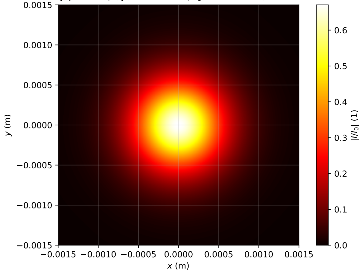
Intensity profile I(x, y, z = 3.742m)/I_0 , \text{Pin}=0.7\text{Pcr} , artificial time
